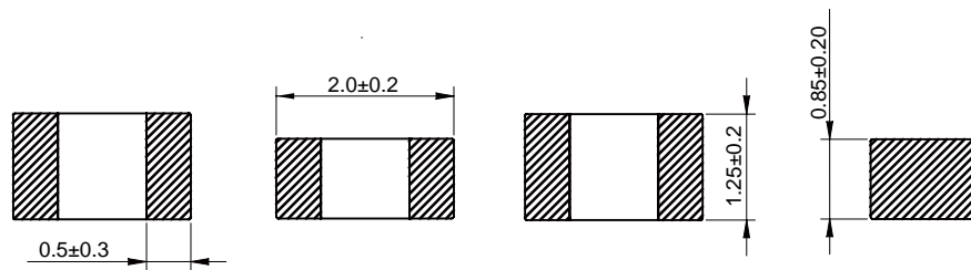
Dimensions: [mm]
